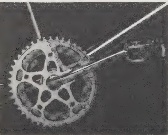
The Browning Automatic Transmission.
